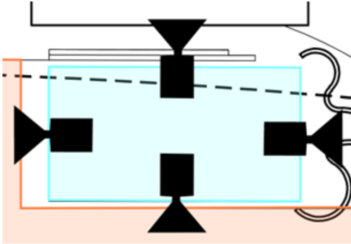
Multi-Sport Courts Illuminance (Fc) Average=7.09 Maximum=15.1 Minimum=2.8 Avg/Min=2.53 Max/Min=5.39
